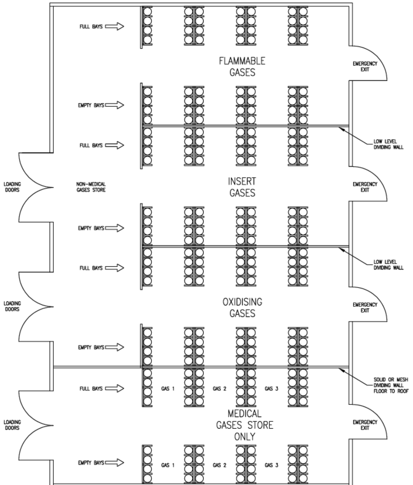
Figure 8.1 - Cylinder storage for medical and non-medical gas cylinders
