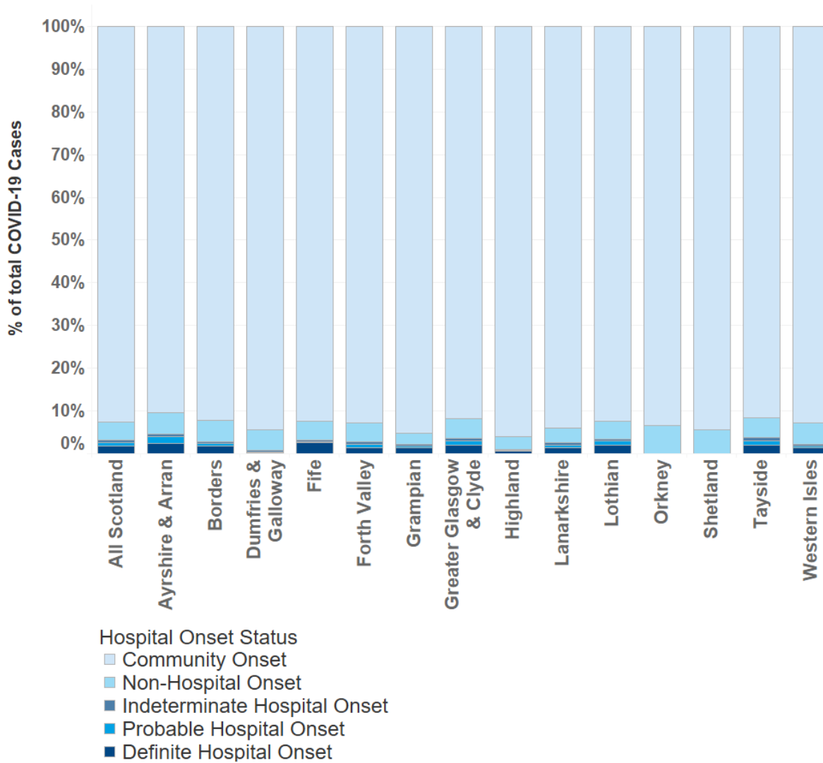
Figure 2: Proportion of COVID-19 cases by onset status and NHS board: specimen dates up to 7 February 2021. 1,2,3
