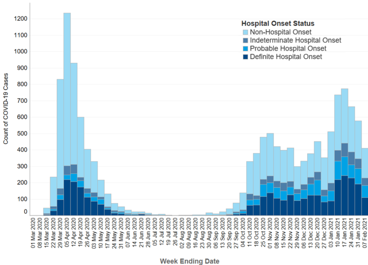
Figure 1: Epidemic curve of COVID-19 cases with first positive specimen taken during an inpatient stay, by onset status: week-ending 1 March 2020 to week-ending 7 February 2021 (n=13,920). 1,2
